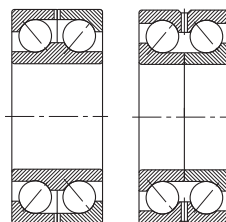
Thrust bearings for wire mills
