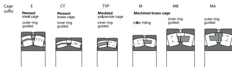
Cages of spherical roller bearings
